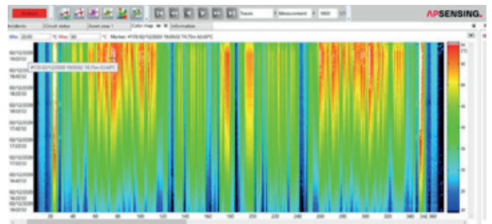
SmartVision displaying busbar temperature color map
